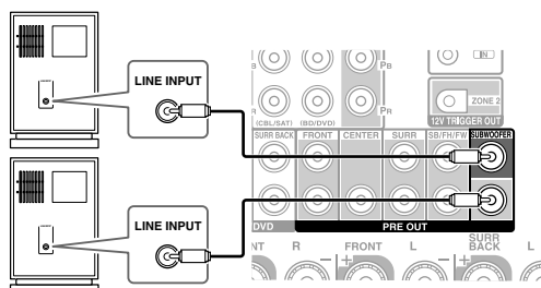
Powered subwoofer
